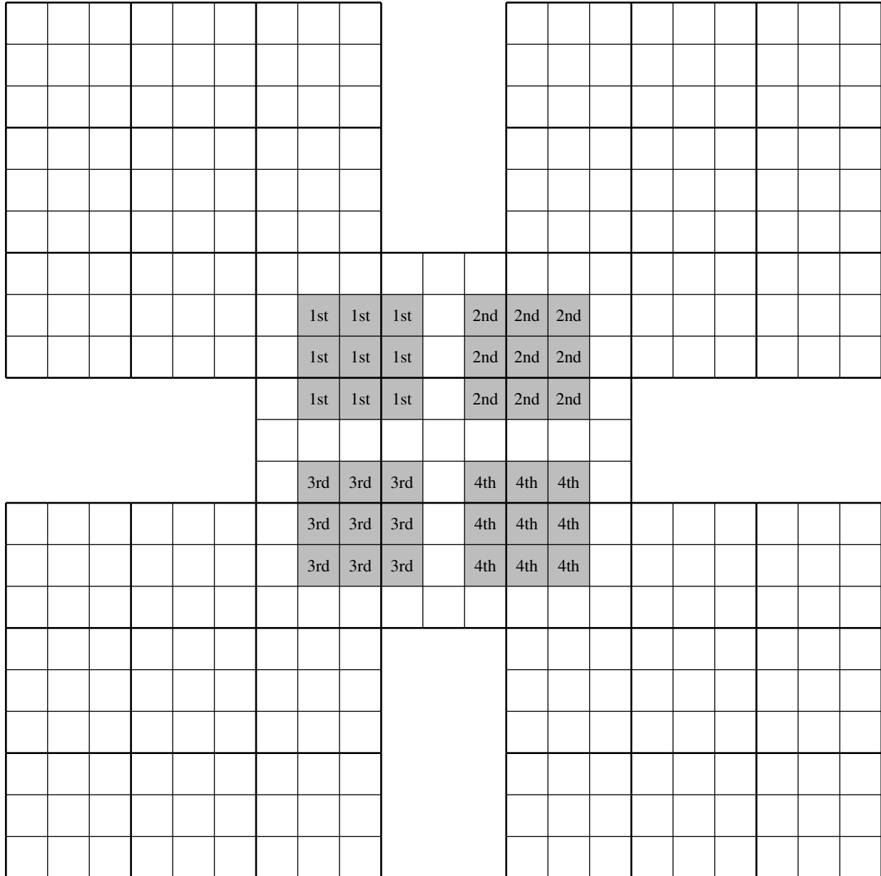
HyperSudoku-by5
